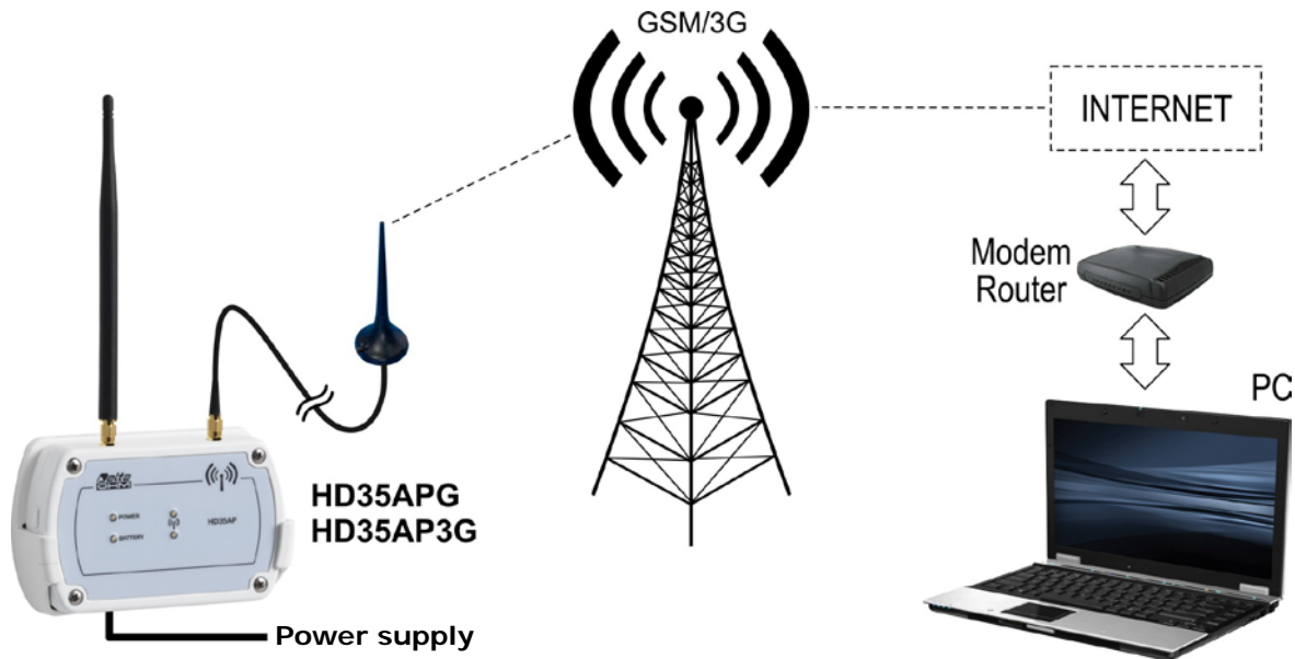
Fig. 6.8.2: GPRS/3G TCP/IP connection
