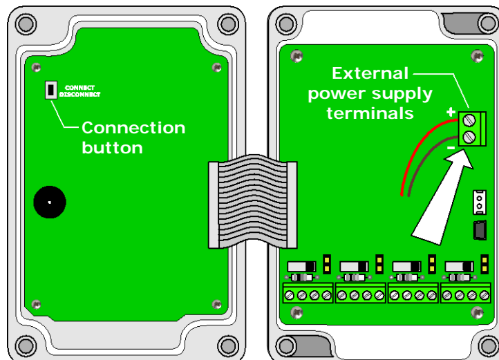
Fig. 9.5.4: connection of the external power supply in the model HD35ED[L]WHE
