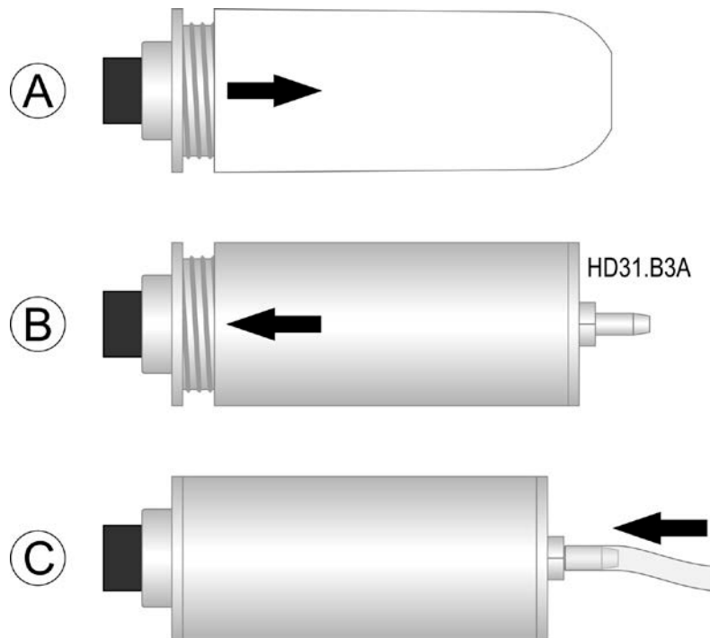
Fig. 9.7.1: CO 2 calibration with cylinder
