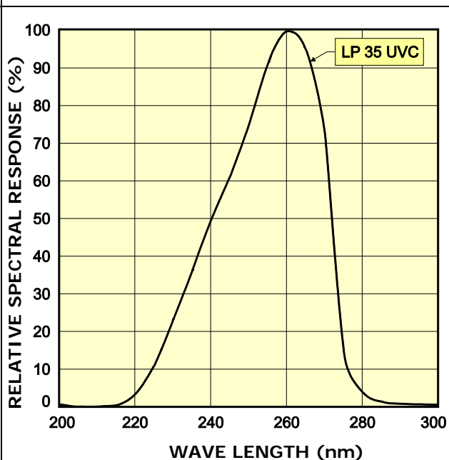
Graph 4 – Relative spectral response of UVC irradiance sensor
