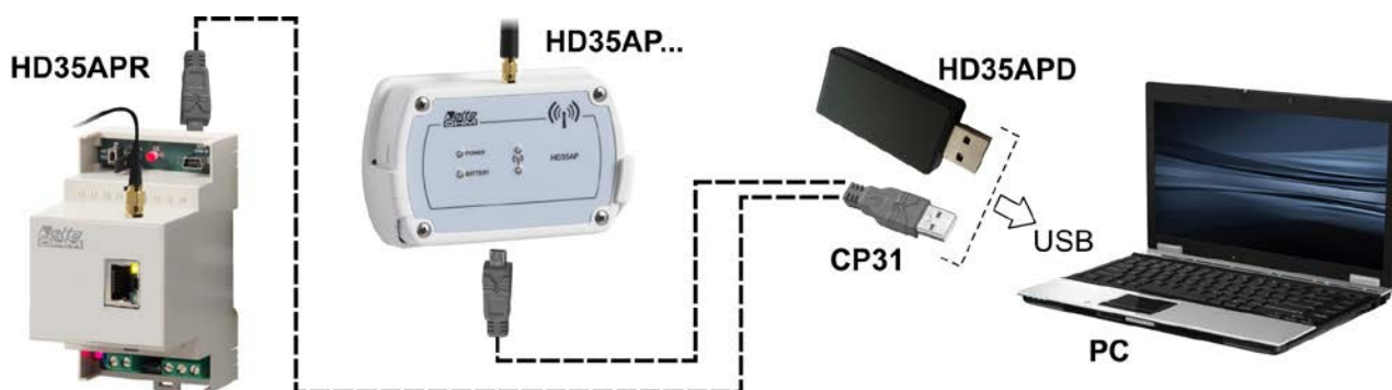
Fig. 6.4.1: USB connection
