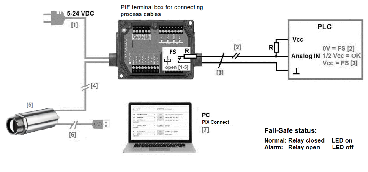
Figure 18: Fail-Safe monitoring states
