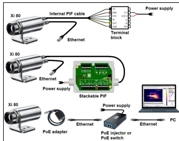
Figure 24: Possibilities of power supply for Xi 80 via Ethernet connection
