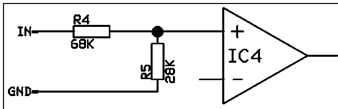
Figure 37: Analog input
