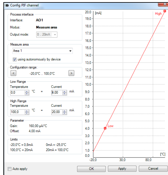
Figure 22: Setup
