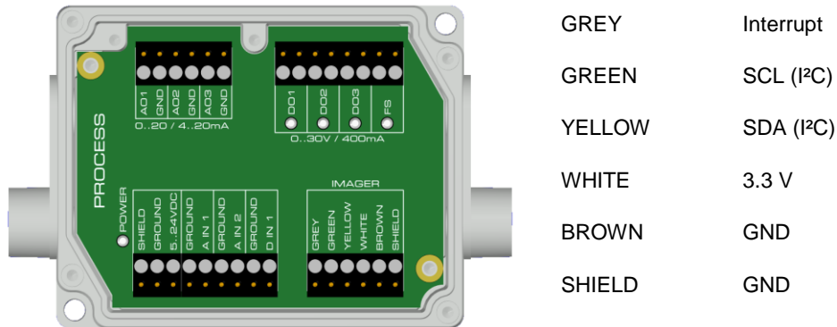
Figure 16: Connections of the industrial Process Interface for Xi 400
