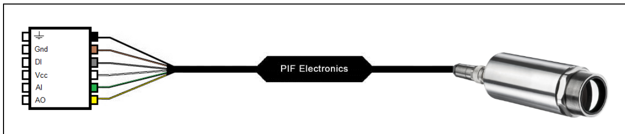
Figure 10: Configuration Standard Process Interface (PIF) Xi 400
