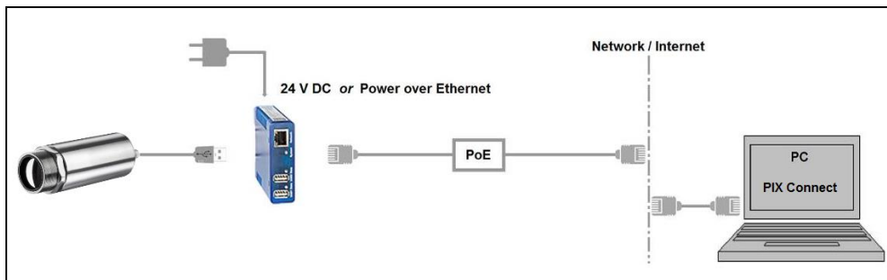
Figure 19: USB Server Gigabit
