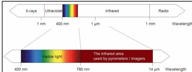
Figure 27: The electromagnetic spectrum and the area used for temperature measurement
