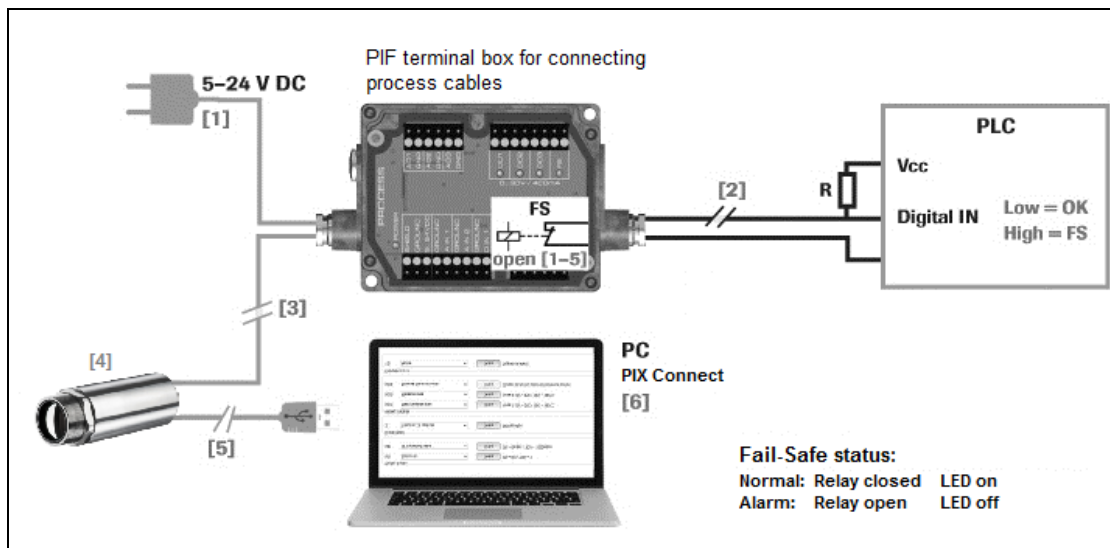
Figure 17: Fail-Safe monitoring states
