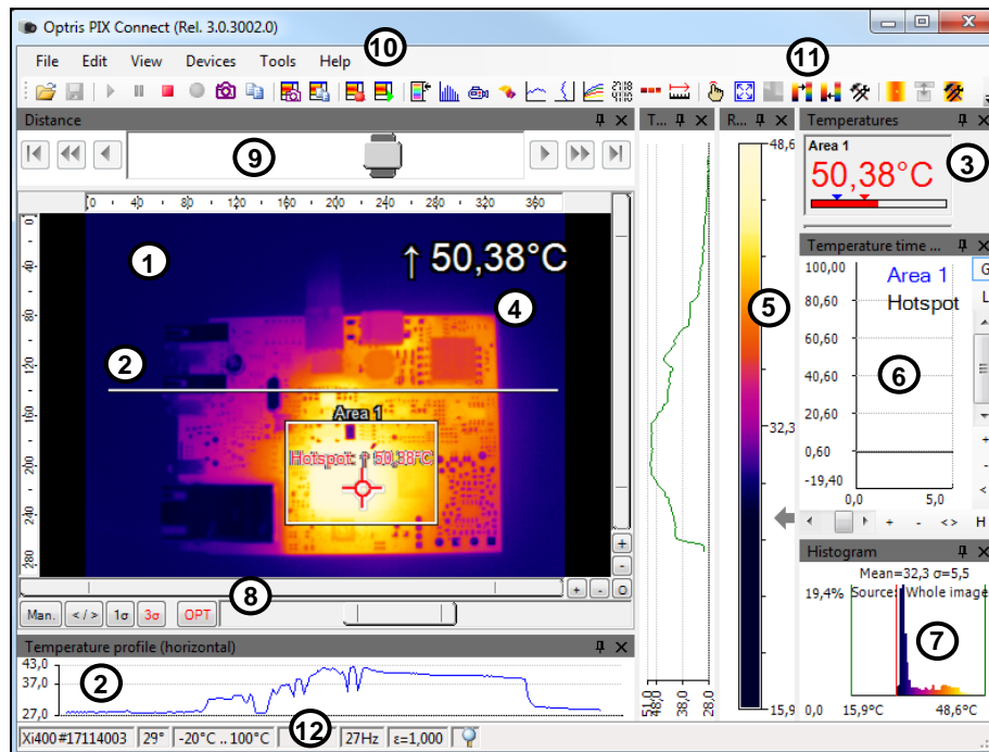
Figure 25: Software window
