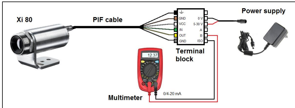
Figure 23: Electrical installation for autonomous operation Xi 80
