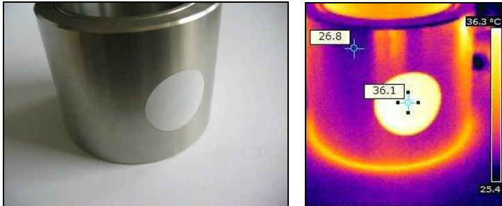
Figure 32: Plastic sticker at metal surface
