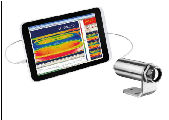
Figure 29: Non-contact thermometry
