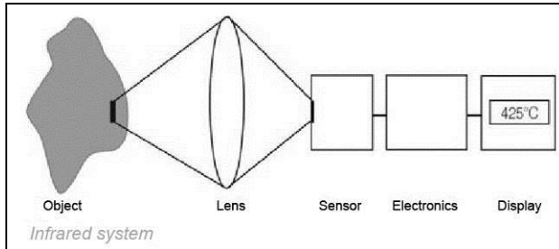
Figure 28: Main principle of non-contact thermometry
