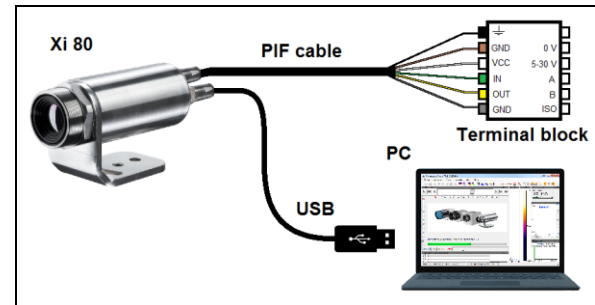
Figure 20: Connection Xi 80 to PC via USB
