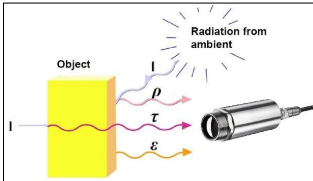
Figure 30: Composition of IR radiation
