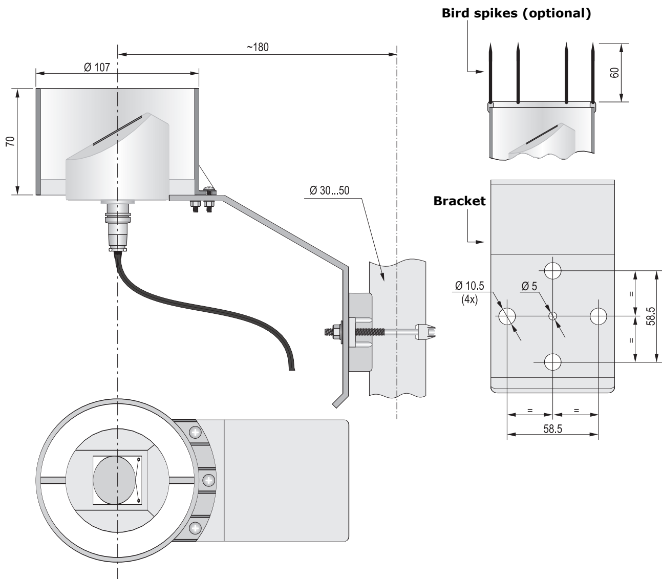
Fig. 2.1: dimensions (mm)
