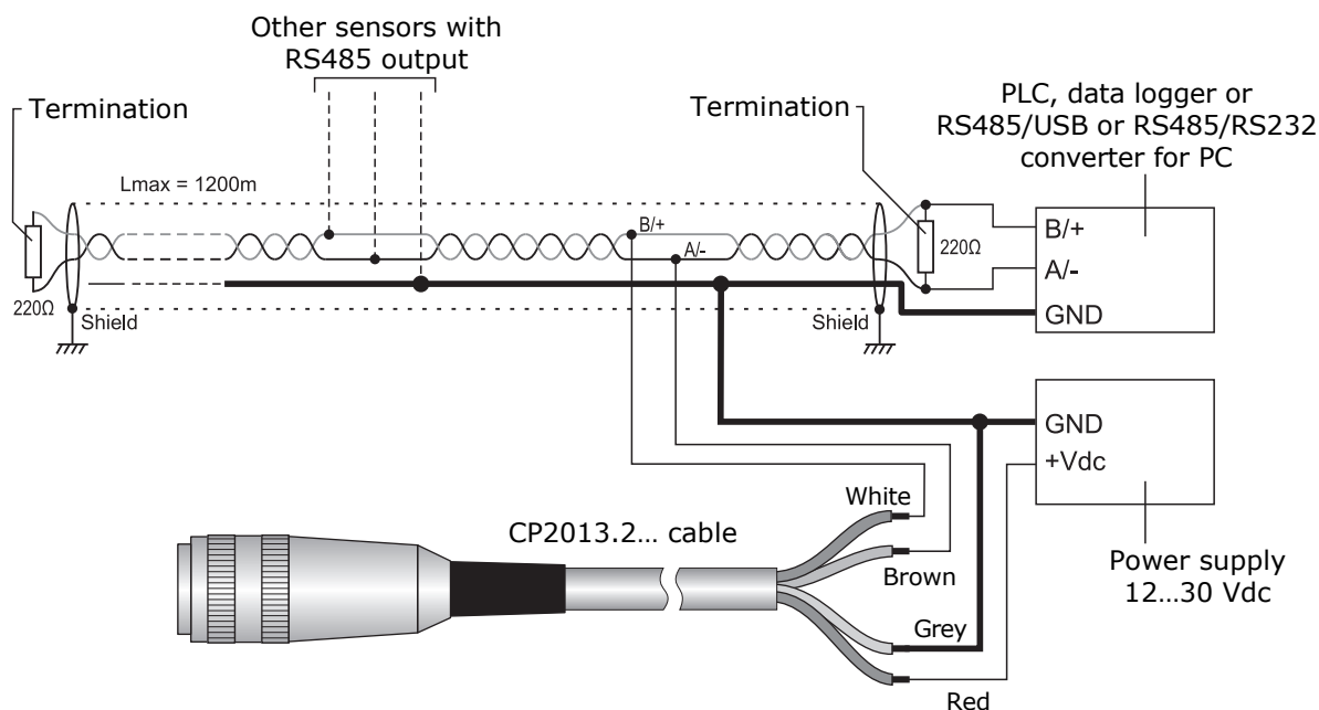
Fig. 3.3: RS485 connection
