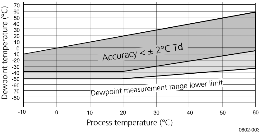
Figure 31 DMP74A Accuracy
