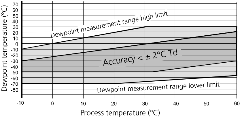
Figure 33 DMP74C Accuracy
