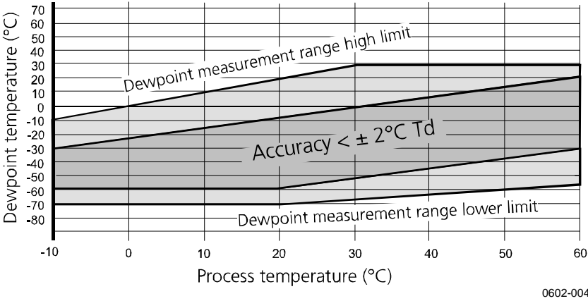
Figure 32 DMP74B Accuracy
