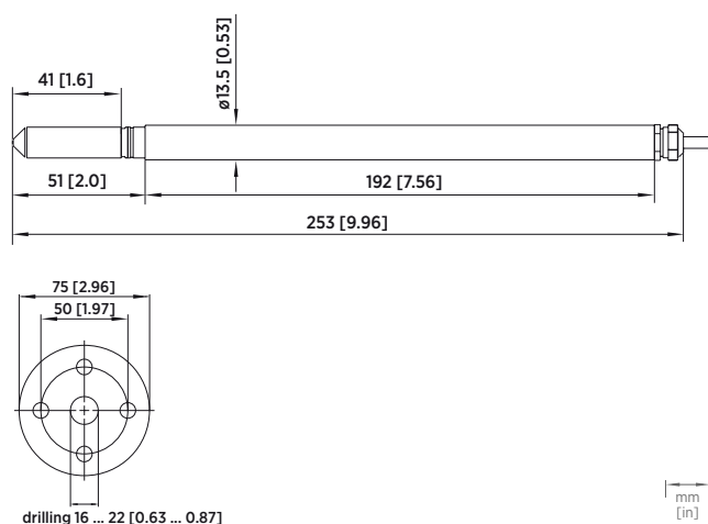
DMP375 probe and stainless steel installation flange dimensions
