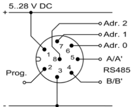
Fig. 3: RS485 connection
