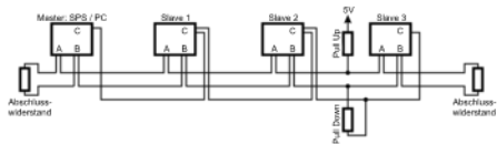
Fig. 2: RS485 communications diagram with terminating resistor Rf
