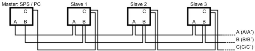
Fig. 1: communications diagram without terminating resistor Rf
