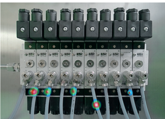
LeakCam 600 with 64 microphones (Power Beam Forming)
