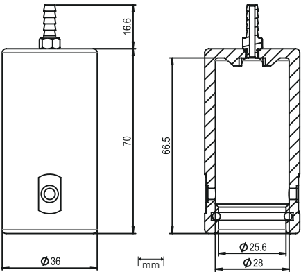
Figure 45 DRW244827SP calibration adapter dimensions
