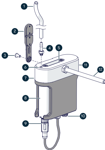
Figure 24 GMP80P probe structure
