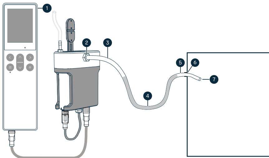
Figure 27 CO 2 sampling from incubator using tube, with GMP80P connected to Indigo80
