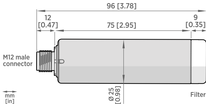
Figure 41 GMP251 dimensions
