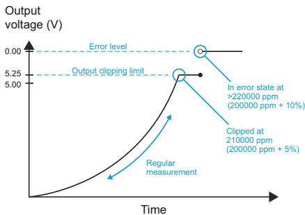
Figure 33 Example of analog output overrange behavior
