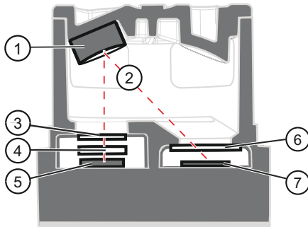
Figure 3 CO 2 measurement in the measurement cuvette
