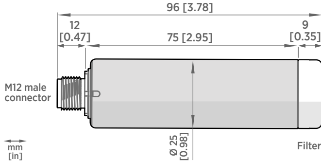
Figure 5 GMP251 dimensions
