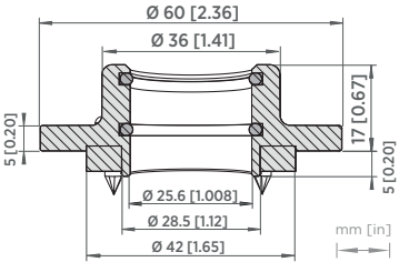
Figure 44 243261SP mounting flange dimensions, cross section
