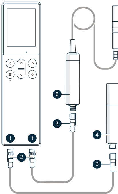
Figure 22 Connecting probes to Indigo80
