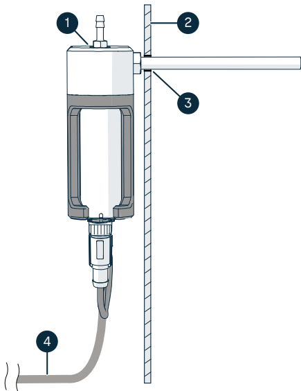
Figure 28 CO 2 sampling from incubator using pipe
