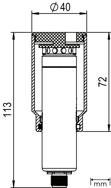
Figure 47 GMP251 spray shield cross section
