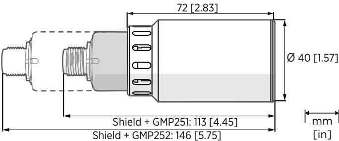
Figure 46 ASM212017SP spray shield dimensions
