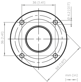
Figure 43 243261SP mounting flange dimensions
