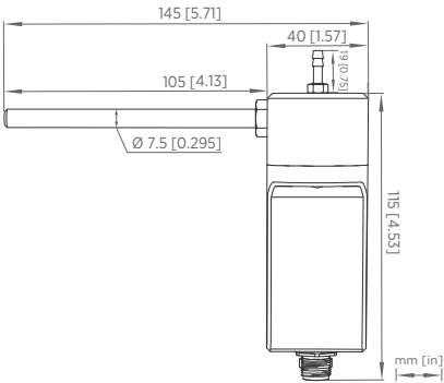
Figure 42 GMP80P dimensions, front and side
