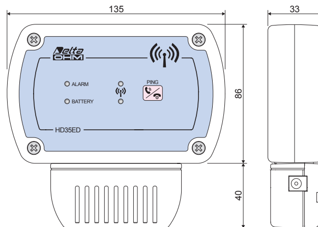
HD35ED... versions with grid
