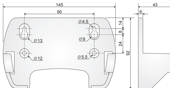
Support for removable installation
