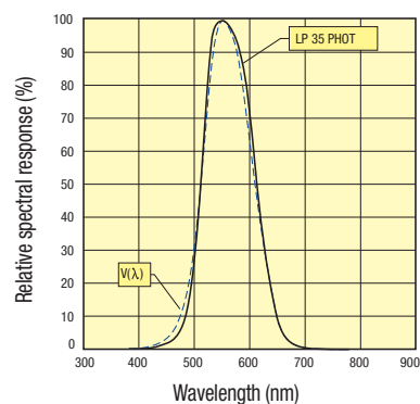
Graph 1 - Relative spectral response of the illuminance sensor
