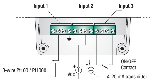
Example of connection of HD35EDH model inputs
