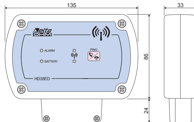
HD35ED... versions with terminal header
