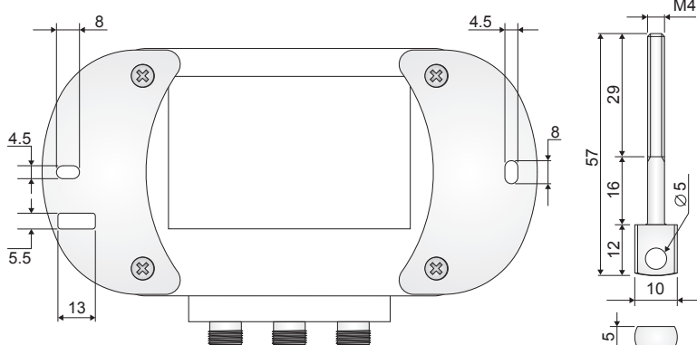
Flanges for fixed installation
