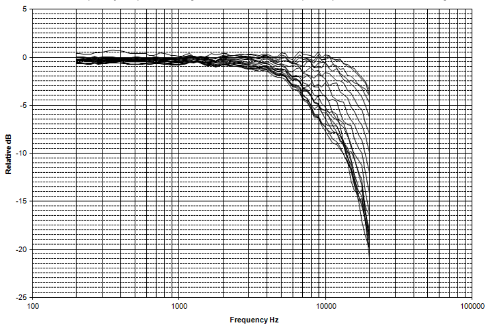
Directional frequency response using windscreen &amp; remote preamp (0°-180° incidence angles)
