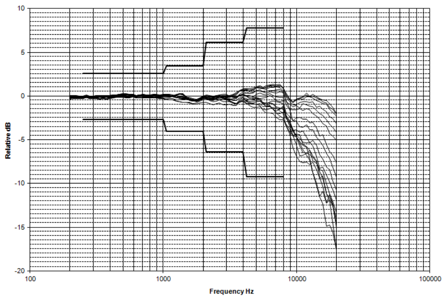
Directional frequency response positioned side toward noise source ( 0^{\circ} - 150^{\circ} incidence angles)
