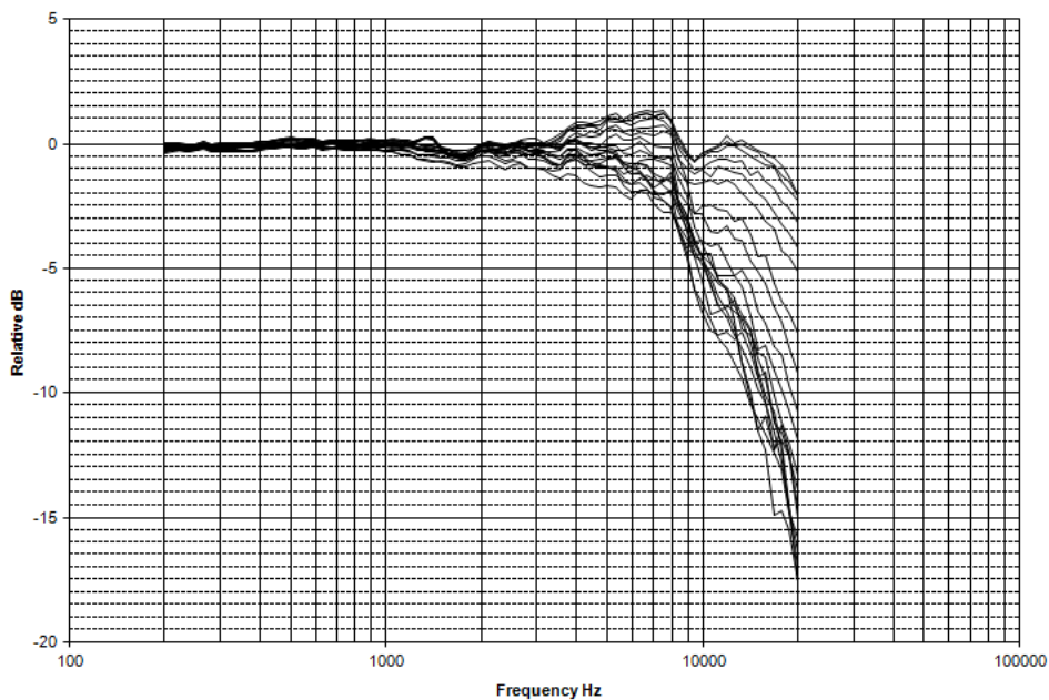
Directional frequency response positioned side toward noise source ( 0^{\circ} - 180^{\circ} incidence angles)
