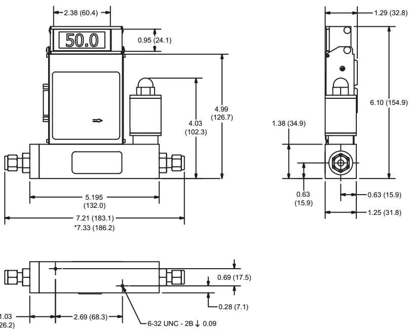
GFC37/47 MASS FLOW CONTROLLER
