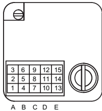
FIGURE 2-3, VALVE CONTROL CONFIGURATION JUMPERS
