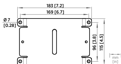
Indigo500 adapter plate dimensions
